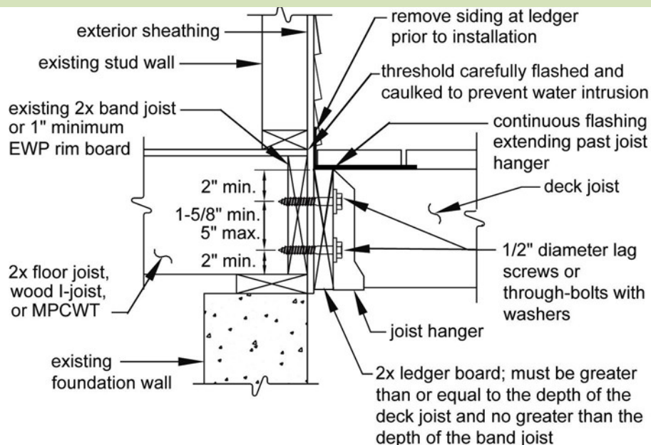
Figure 10. General Attachment of Ledger Board to Band Joist or Rim Board
